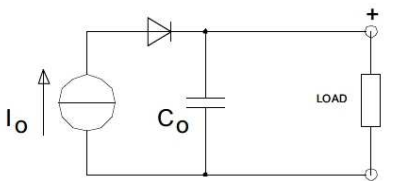
Conventional power supply circuit simplified, without PSINK
