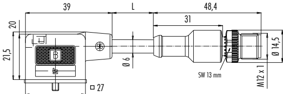
Connecting cable female power connector – male cable connector M12
