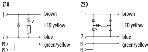
Connecting cable female power connector, wired, LED – male cable connector M12
