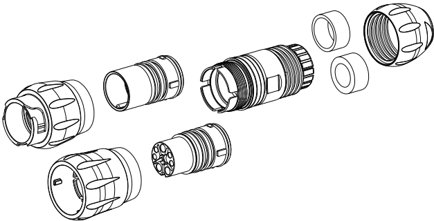
Flat seal enclosed loose
