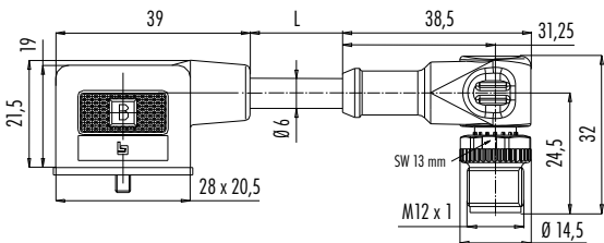
Connecting cable female power connector – Male angled connector M12
