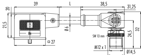
Connecting cable female power connector, wired, LED – male angled connector M12
