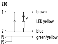
Connecting cable female power connector, wired, LED – male angled connector M12
