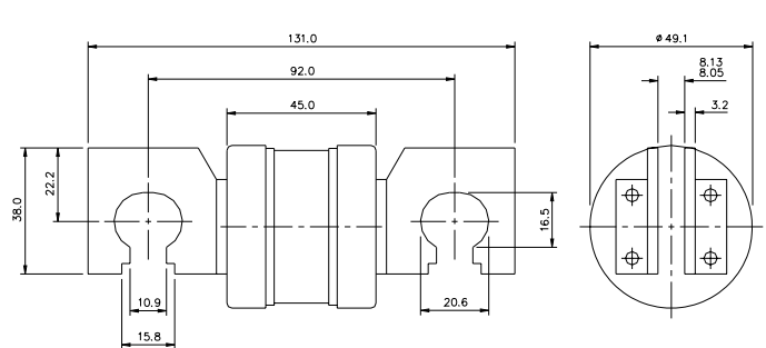
Dimensions for SJ28
