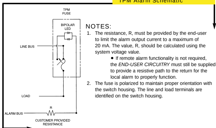
TPM Alarm Schematic
