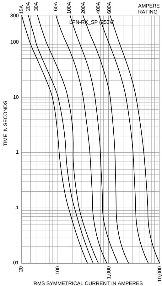
Time-Current Characteristic Curves—Average Melt
