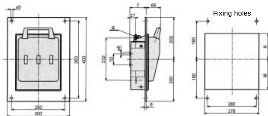
Fuse switch-disconnector LBS4a with shield for front fixing
