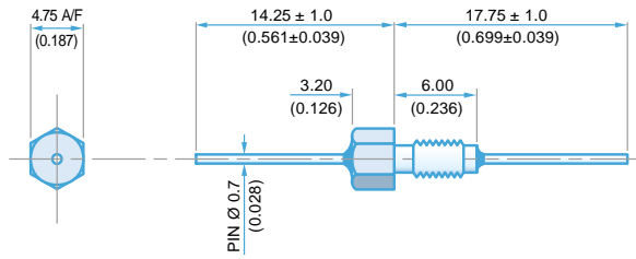
8-32 UNC Class 2A Thread 4.75mm Hexagonal Head
