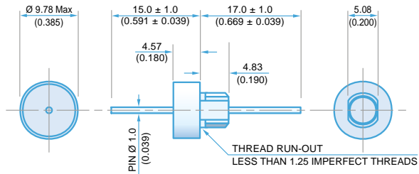
¼-28 UNF Class 2A Thread 9.8mm Round Head
