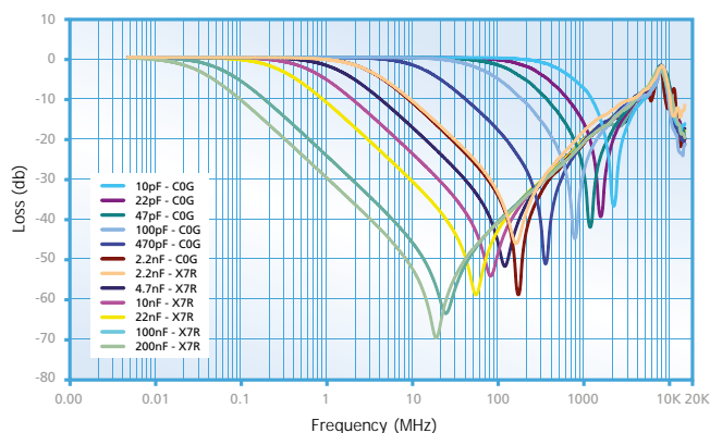
E01 &amp; E07 Insertion Loss
