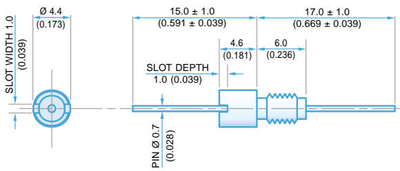
6-32 UNC Class 2A Thread 4.4mm Round Head
