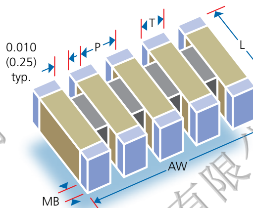
Dimensions - inches/mm
