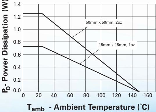
Derating curves
