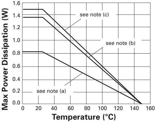
Derating curve
