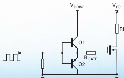
Figure 3. Totem-pole driver stage for power MOSFET
