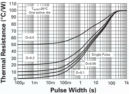
Derating curves
