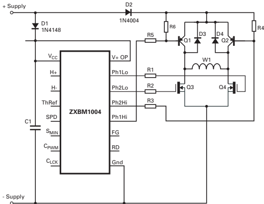
Figure 5. Single-phase fan motor circuit
