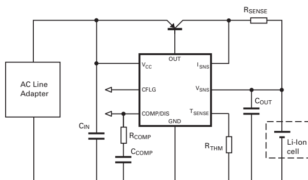
Figure 2. A typical linear charger circuit
