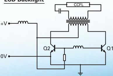
LCD Backlight
