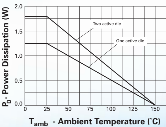
Derating curves
