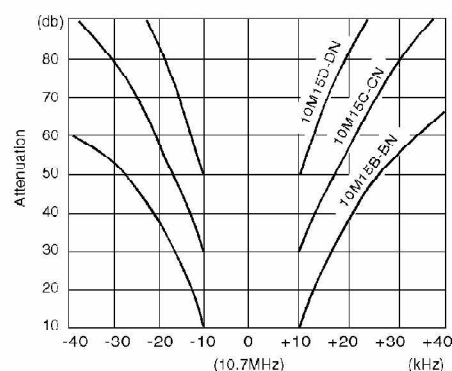
MULTI-POLE CHARACTERISTICS
