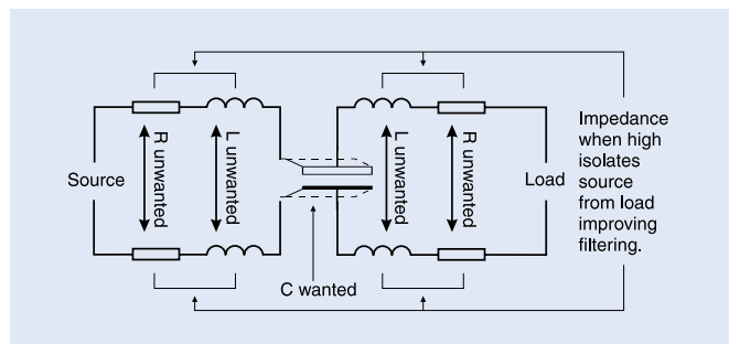
Figure 2: T-Network capacitor
