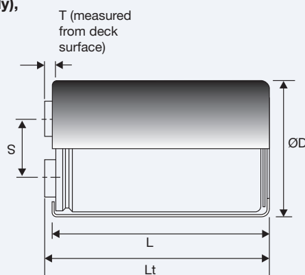
ALS40 Clamp Mounting
