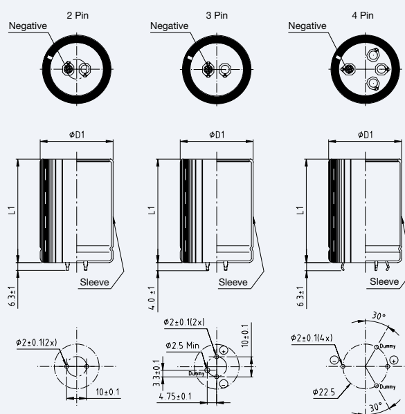
Pin Configuration
