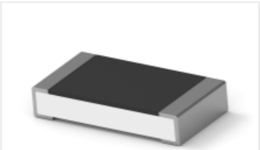
TE Part #6-2176389-5 RQ 1206 499R 0.1% 10PPM 5K RL
