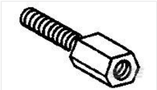
TE Part #5747404-3 FEMALE SCRLOCK,METRIC,ZN PLTD
