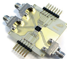
CHC6094-QKB in QFN 4x4
