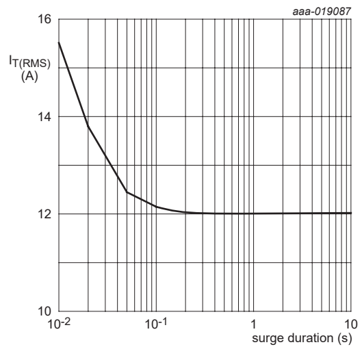
f = 50 Hz; T_{mb} = 121\text{ °C} Fig. 2. RMS on-state current as a function of surge duration; maximum values
