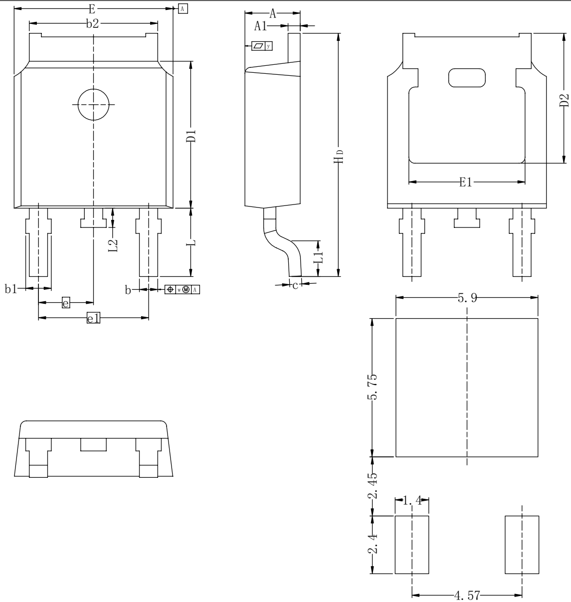
Recommended Footprint
