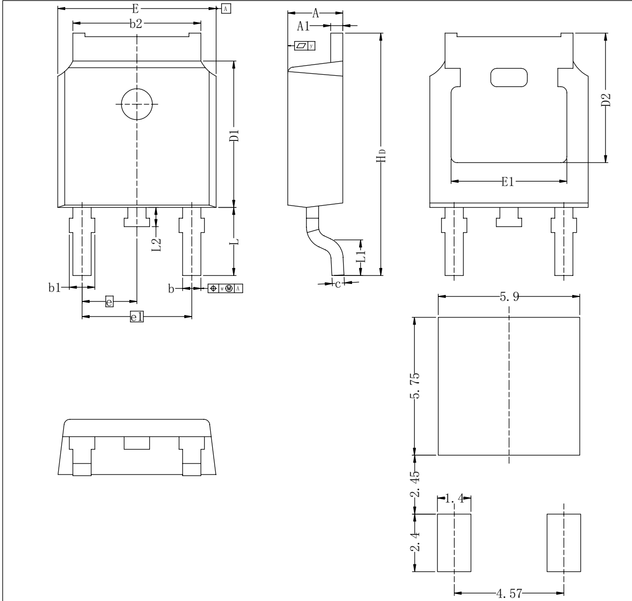
Recommended Footprint
