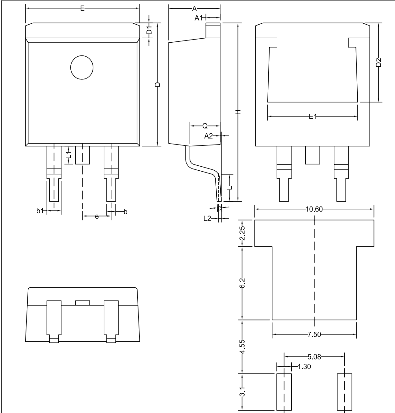
Recommended Footprint
