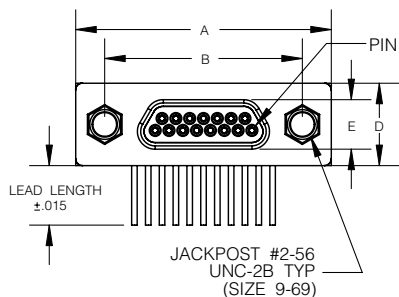
PLUG
