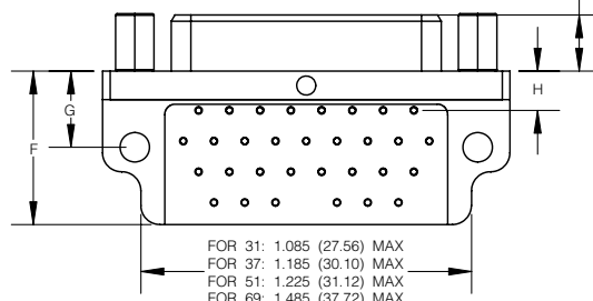
VIEW SHOWN FOR 31, 37, 51 and 69 CONTACT ARRANGEMENTS
