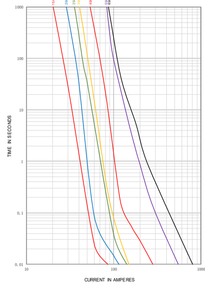
Average Time Current(I-T Curves)
