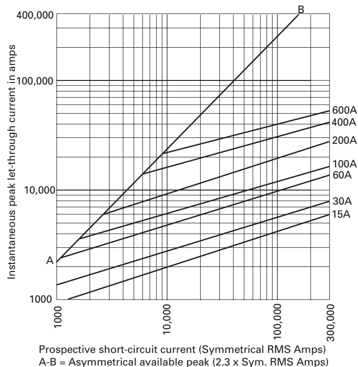
LPS Current limitation curves
