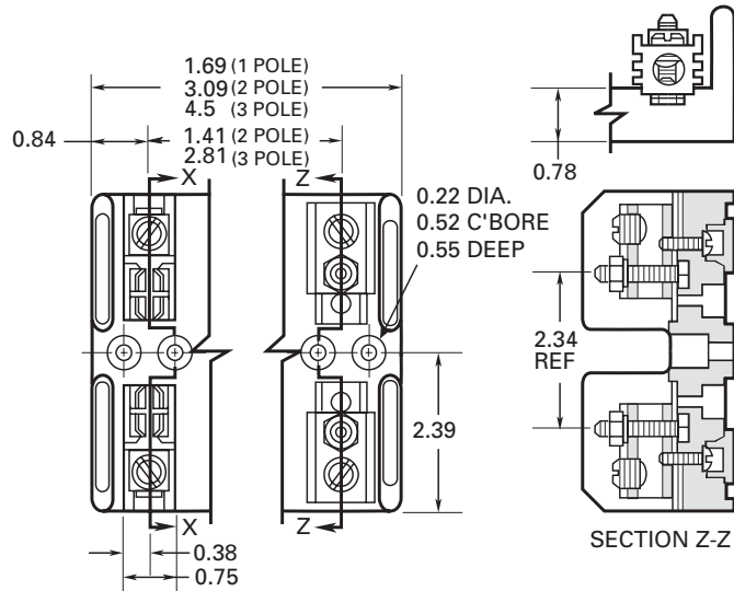
Figure 3. 61 to 100 A
