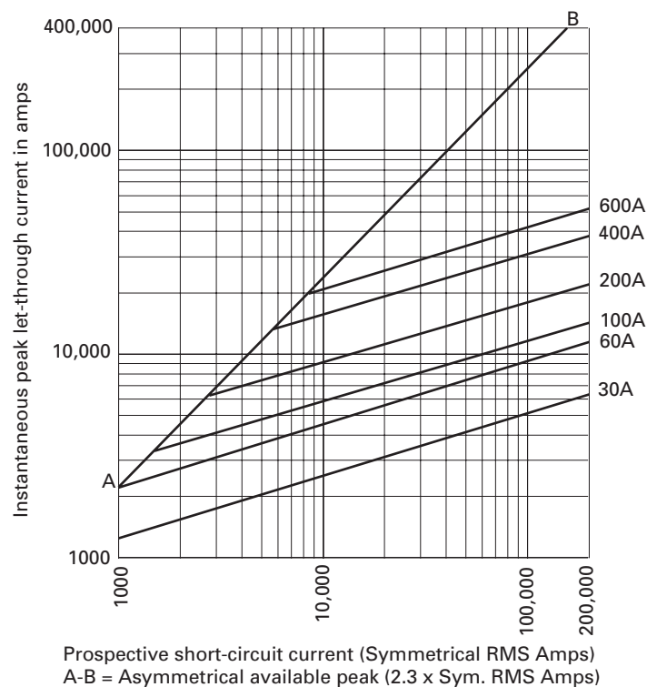
LPN Current limitation curves
