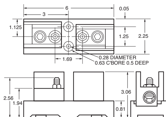
Figure 3. 101 to 200 A
