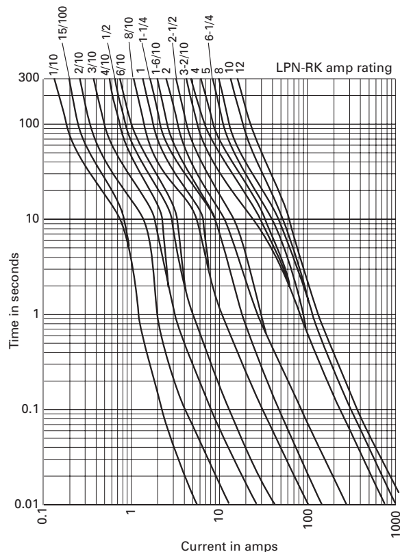
LPN Time-current characteristics — average melt
