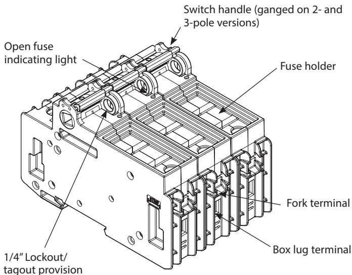
Left side Uses counterclockwise handles
