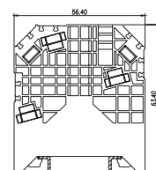
Dimensions — mm
