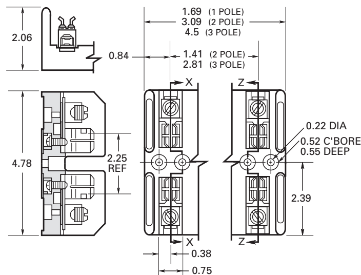
Figure 2. 61 to 100 A
