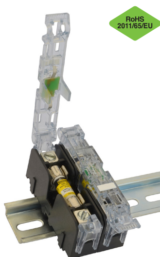
BPVM-2C with CVRI-CCM covers
