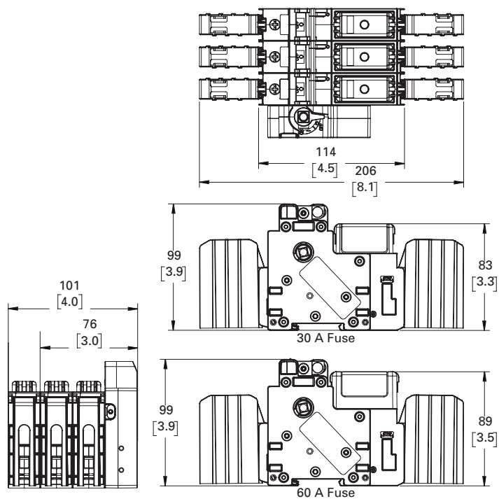
Left front rotary switches (shown with optional terminal shrouds)
