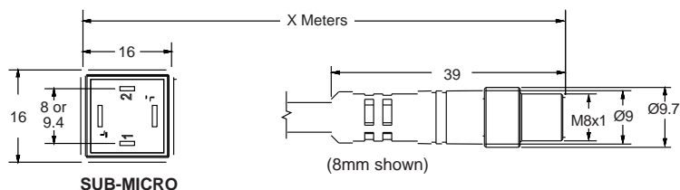
8mm Male Input
