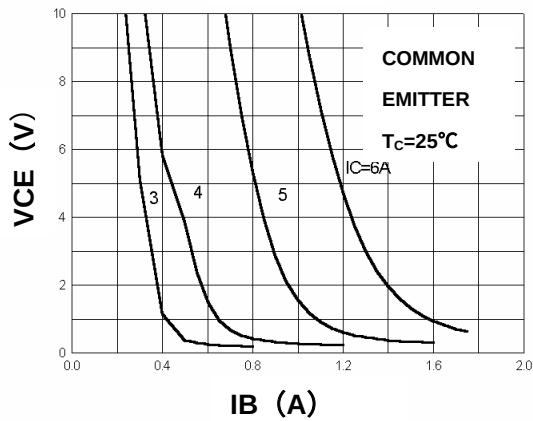
VCE – IB
