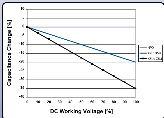
Voltage Coefficient
