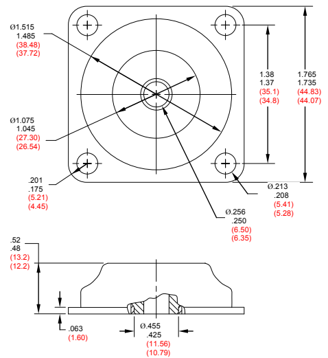
FIGURE 1 – PART DIMENSIONS
