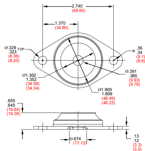
FIGURE 1 – PART DIMENSIONS
