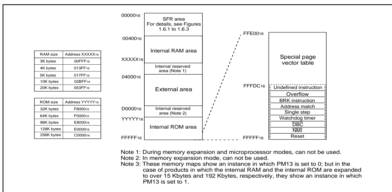
Figure 1.3.1. Memory map
