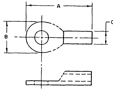
TERMINALS FOR WIRE SIZES 12 TO 0000
