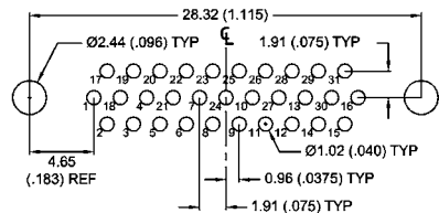
31 CONTACTS - VIEW A
