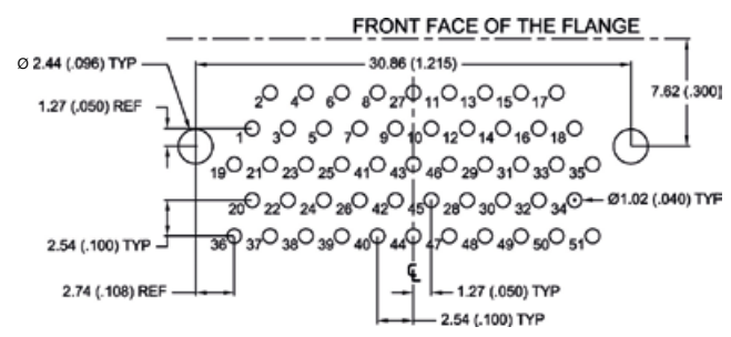
51 CONTACTS - VIEW B
