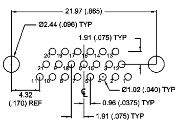
21 CONTACTS - VIEW A
