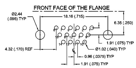
15 CONTACTS - VIEW B
