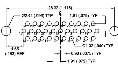
31 CONTACTS - VIEW A
