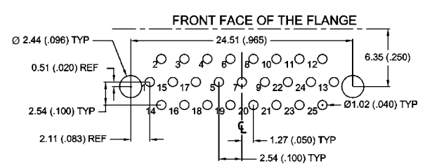
25 CONTACTS - VIEW B
