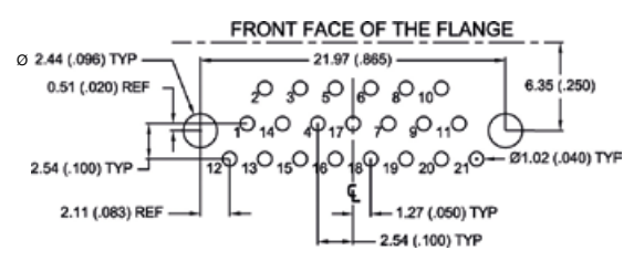
21 CONTACTS - VIEW B
