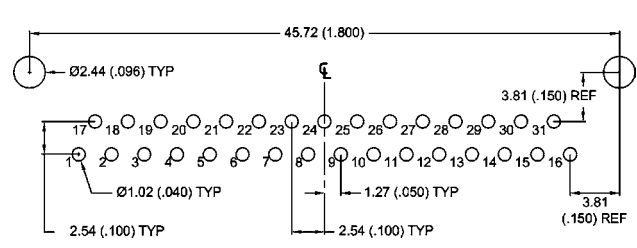
31 CONTACTS - VIEW B
