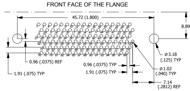
100 CONTACTS - VIEW B
