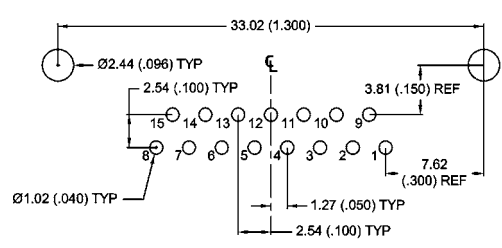
15 CONTACTS - VIEW B
