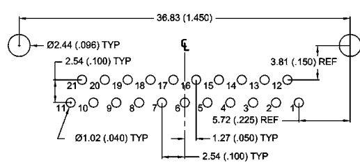
21 CONTACTS - VIEW B
