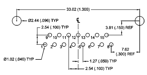
15 CONTACTS - VIEW B
