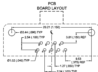
9 CONTACTS - VIEW B
