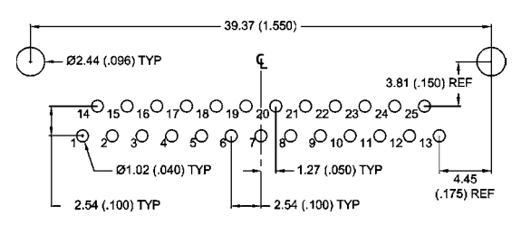
25 CONTACTS - VIEW B
