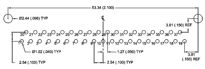
37 CONTACTS - VIEW B
