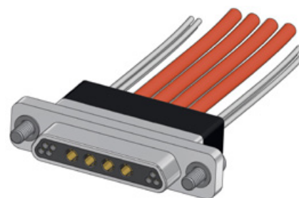
4 POWER COMBO CONTACTS + 7 SIGNALS
