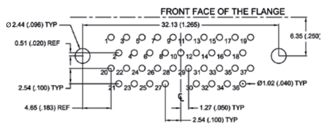
37 CONTACTS - VIEW B
