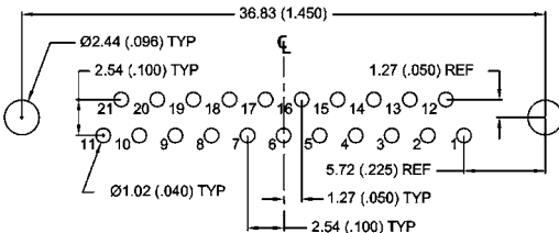
21 CONTACTS - VIEW ALL
