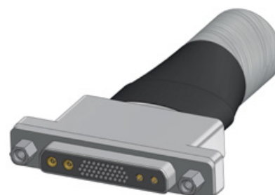
2 POWER COMBO S2.2 + 2 COAXIAL COMBO S3 CONTACTS + 40 SIGNALS, INTEGRATED IN A HARNESS
