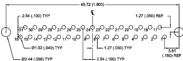
31 CONTACTS - VIEW ALL
