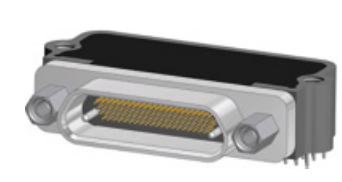
CONDENSED BOARD RIGHT ANGLE TYPE (CBR) 0.050" PITCH
