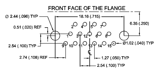
15 CONTACTS - VIEW B
