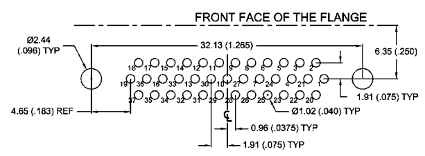
37 CONTACTS - VIEW B
