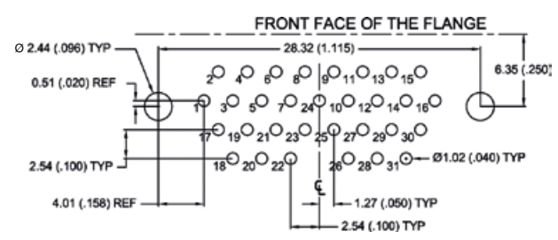
31 CONTACTS - VIEW B
