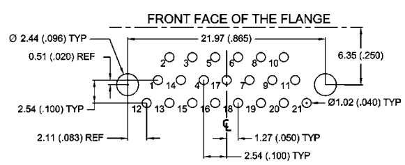
21 CONTACTS - VIEW B
