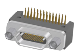
CONDENSED BOARD RIGHT ANGLE TYPE (CBR) 0.050" PITCH
