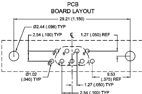
9 CONTACTS - VIEW ALL
