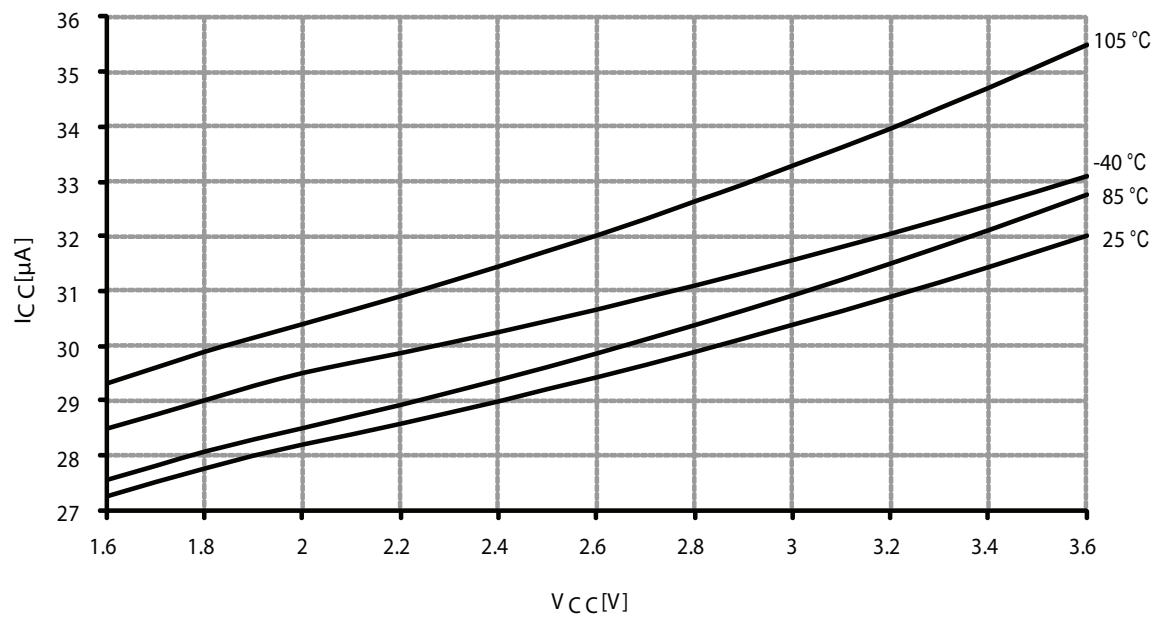
Figure 37-10. Idle mode supply current vs. V_{\text{CC}} .
