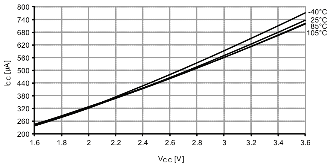
Figure 37-253. Active mode supply current vs. V_{CC} .
