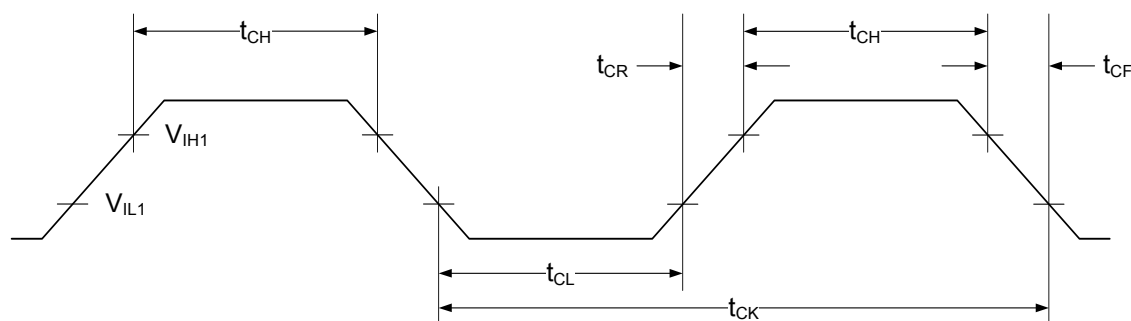
Figure 36-3. External clock drive waveform
