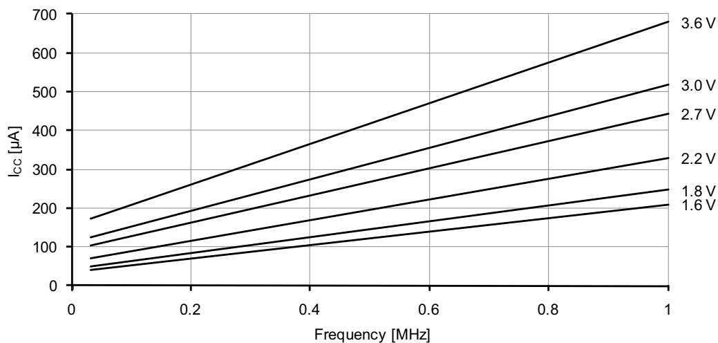
Figure 37-2. Active supply current vs. frequency.
