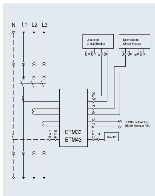
Three-pole circuit-breaker with ETM33/ETM43 electronic release (External natural current transformer)
