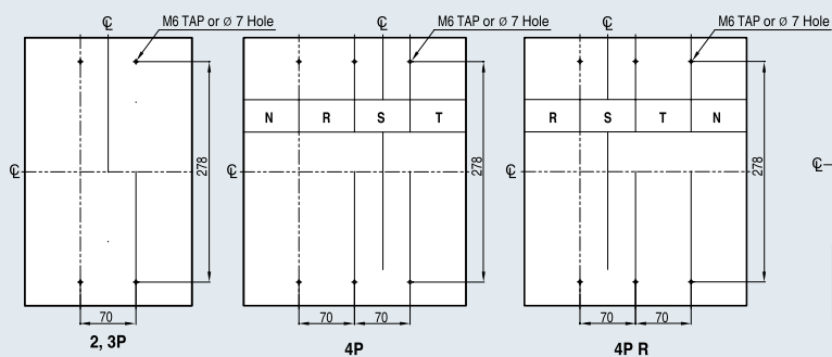
Panel drilling
