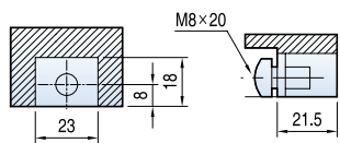
Terminal section
