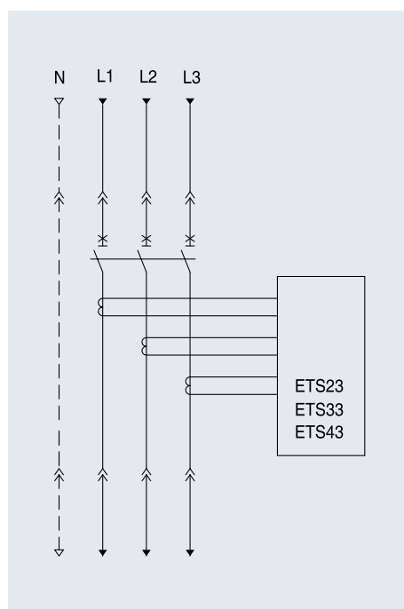
Three-pole circuit-breaker with ETS23/ETS33/ETS43 electronic release
