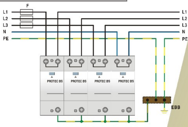
TN-S Network (V-connection)
