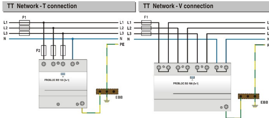
Connection diagram
