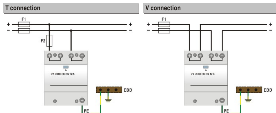
Connection diagram
