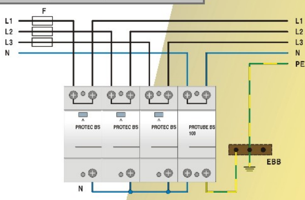
TT Network (V-connection)
