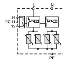
Connection diagram
