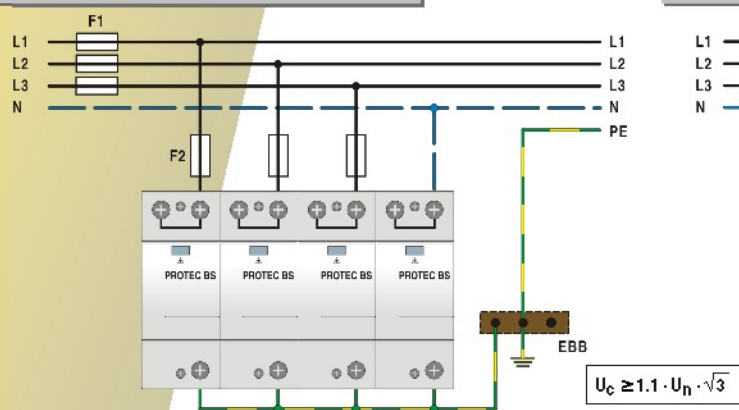
IT Network (T-connection)
