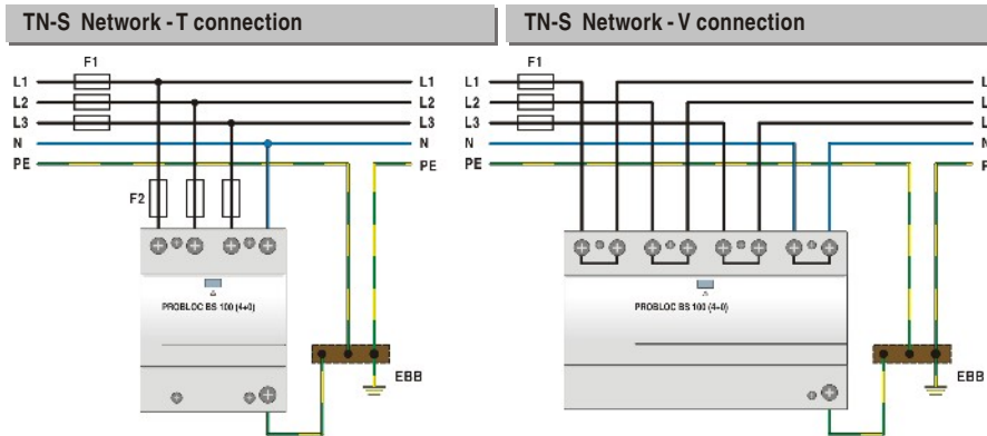
Connection diagram
