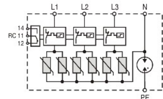
Connection diagram
