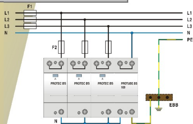
TT Network (T-connection)
