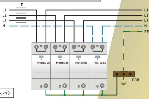
IT Network (V-connection)
