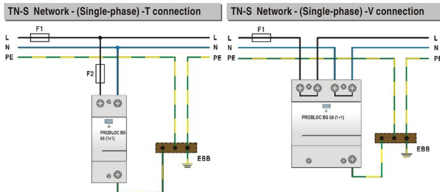
Connection diagram
