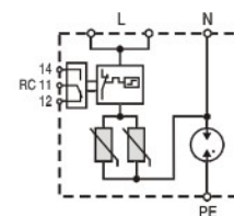
PROBLOC BSR 50/xxx (1+1)
