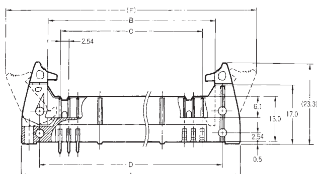
Straight DIP terminals
