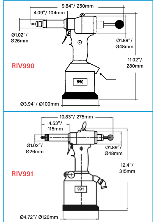
RIV990 (2986300 tool only) Cuts hex hole sizes for #8 to 5/16" and M4 to M8
