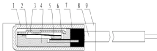
KSD Series structure(metal casing)
