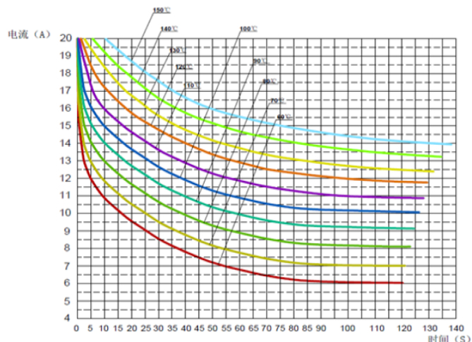
Current vs. Tripping time
