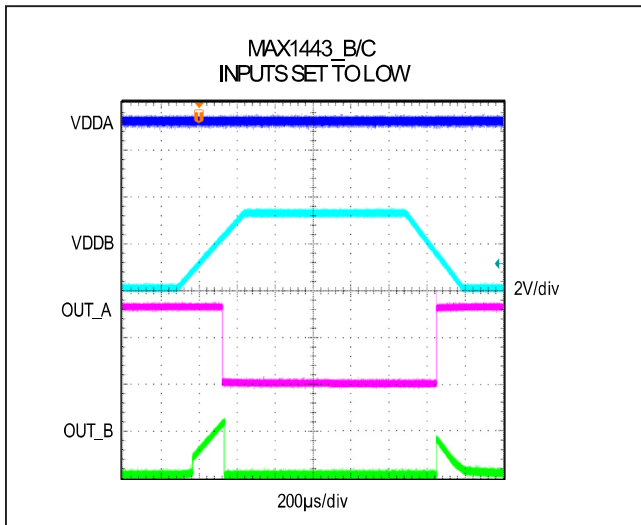
Figure 7. Undervoltage Lockout Behavior (MAX1443_B/C Low)
