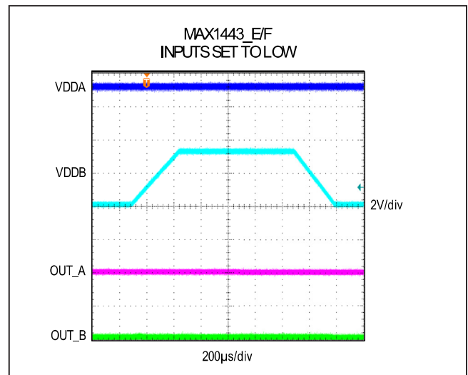
Figure 8. Undervoltage Lockout Behavior (MAX1443_E/F Low)
