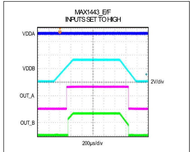
Figure 6. Undervoltage Lockout Behavior (MAX1443_E/F High)
