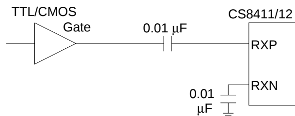
Figure 24. TTL/CMOS Interface
