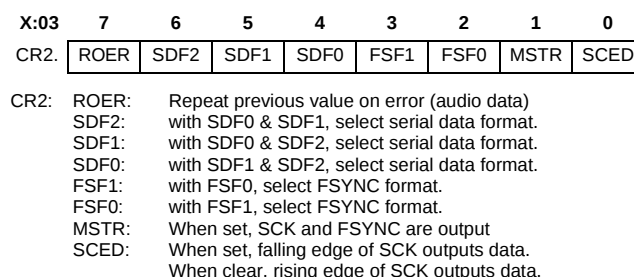
Figure 9. Control Register 2
