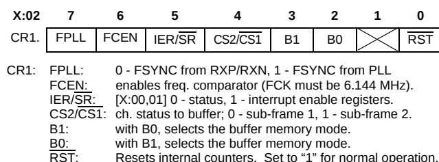
Figure 8. Control Register 1
