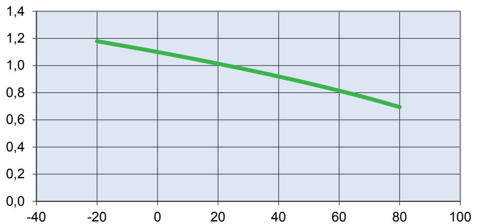
CH10x85 gPV Temperature Derating Factor
