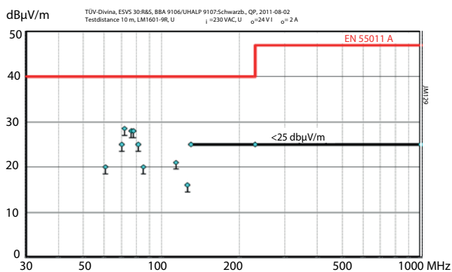
Fig. 14b Typical radiated emissions of LM1601-9R according to IEC/EN 55011/32, normalized to a distance of 10 m, measured at V i = 230 VAC and I o nom .
