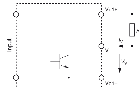
Fig. 24 Output configuration of options V0, V2, V3
