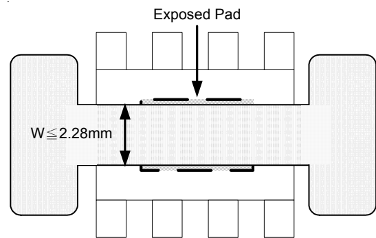
Figure 11. Dog-Bone Layout
