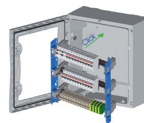
Simply wire and "Click it in"
