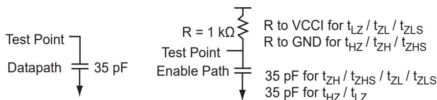
FIGURE 2-9: AC LOADING
