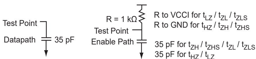
FIGURE 2-10: AC LOADING
