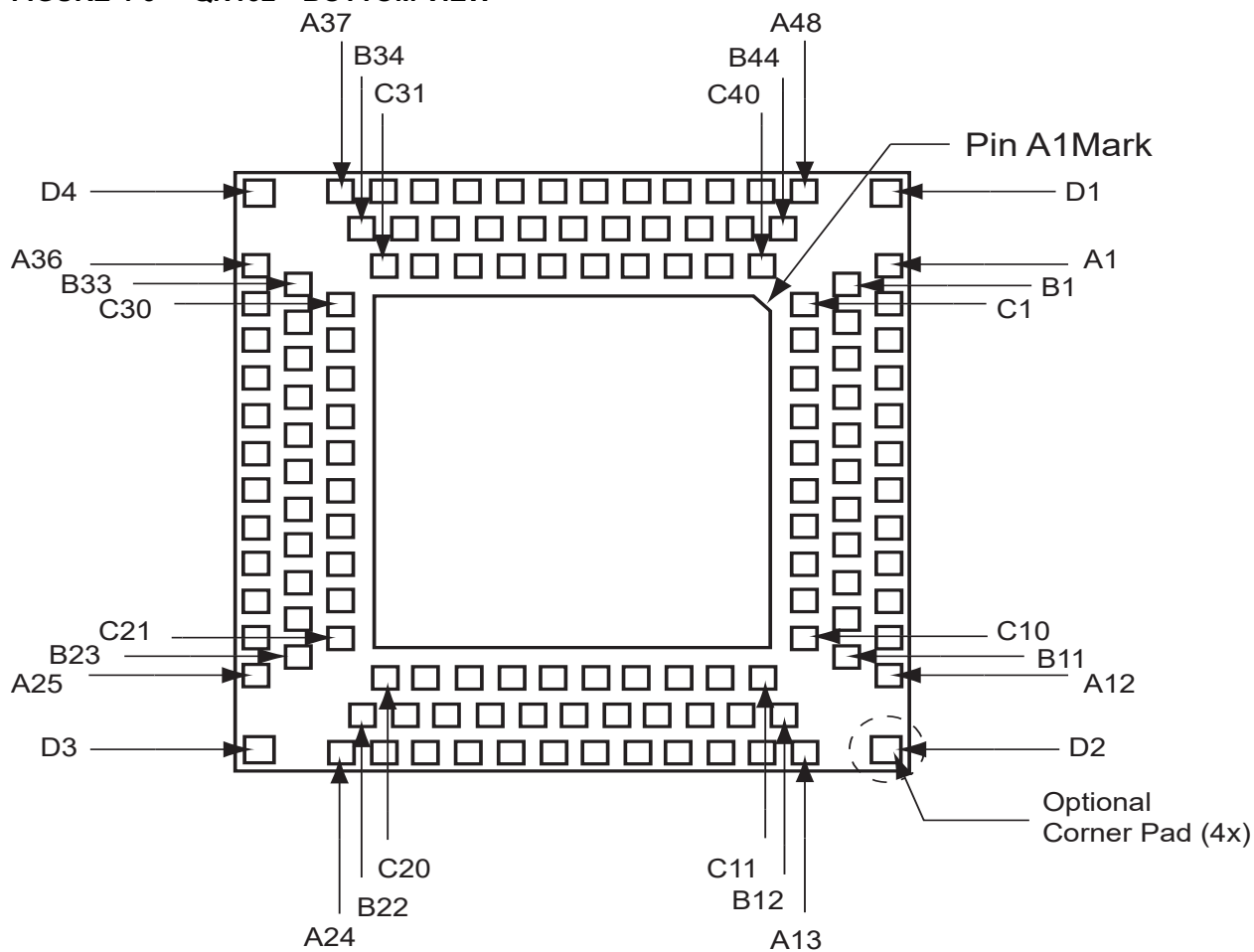
FIGURE 4-3 • QN132—BOTTOM VIEW
